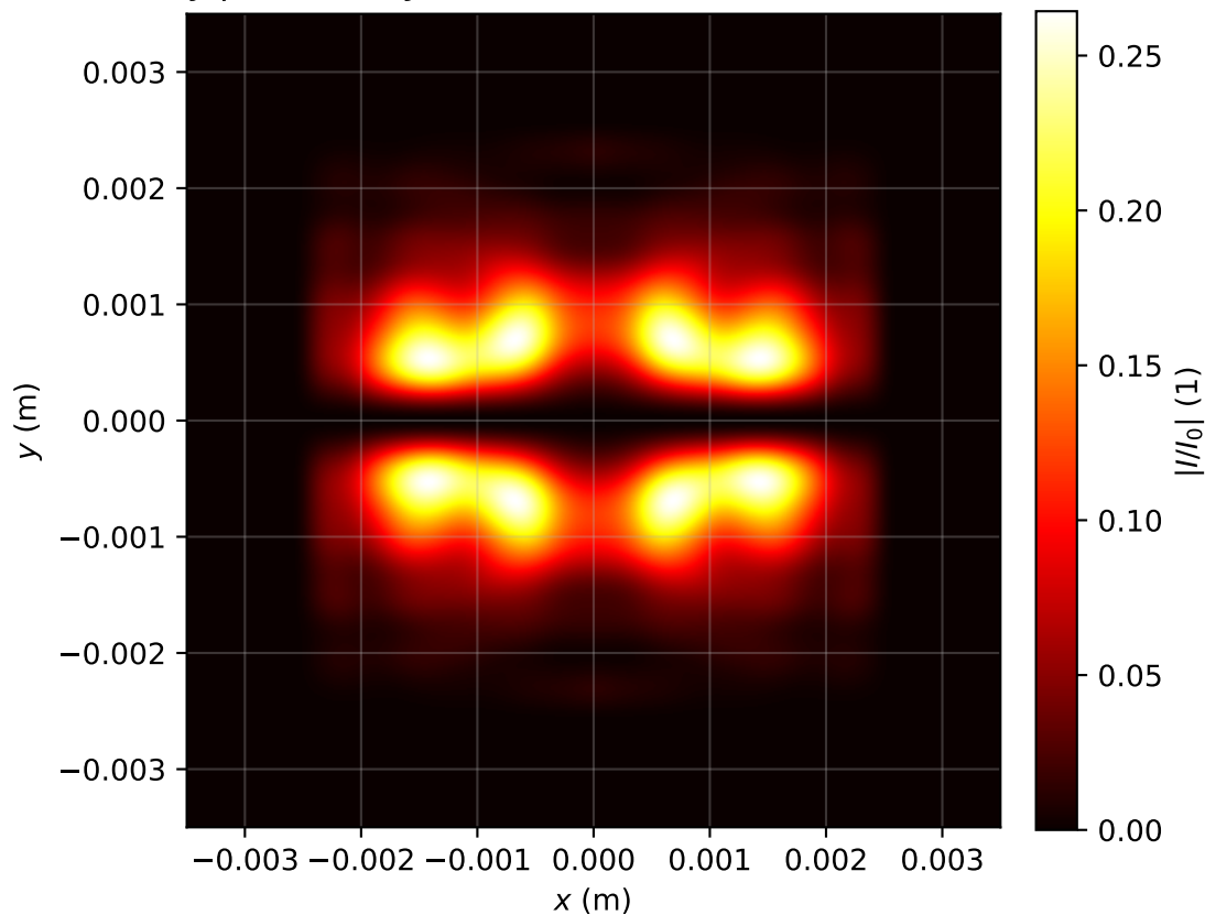
Intensity profile I(x, y, z = 3.503)/I_0 , P_{in}=4.0P_{cr} , artificial time
